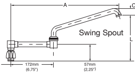
GROUP NO. 4 Double Joint
